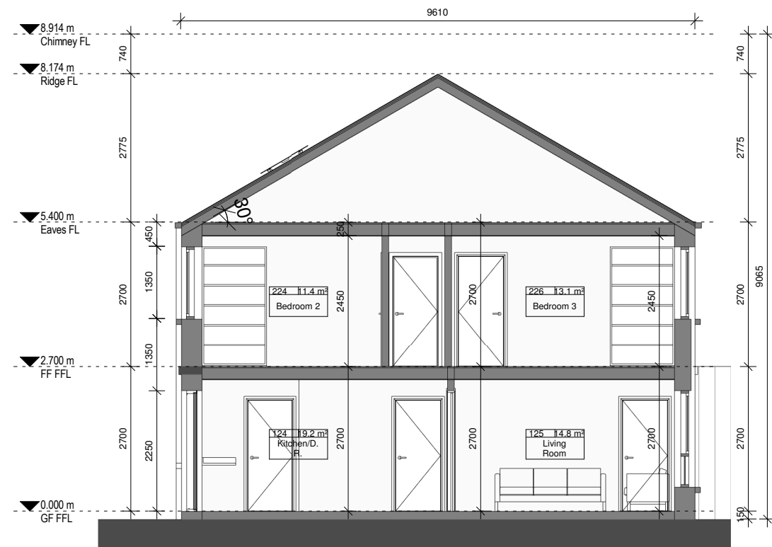
1 Section 1 1 : 100 @ A3
